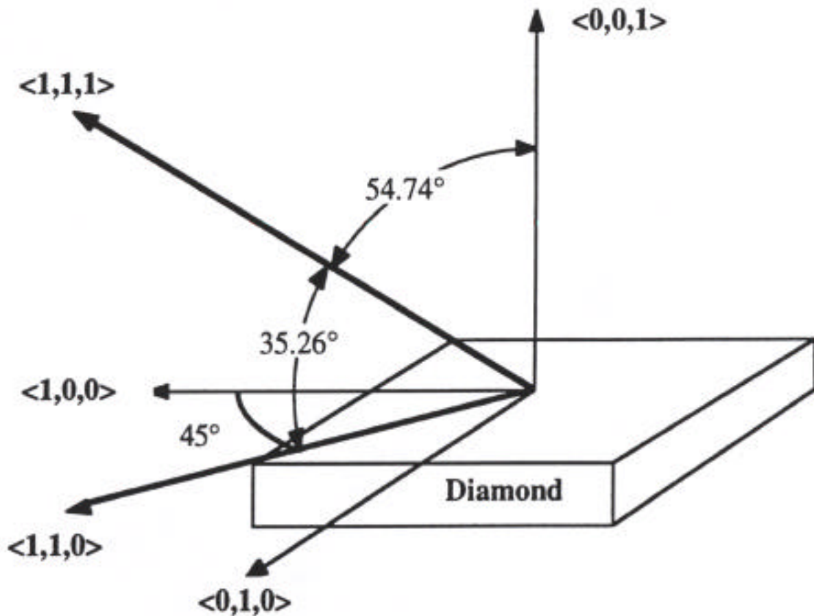
Figure 3.5. Orientation of \langle 111 \rangle and \langle 110 \rangle conventional cubic cell reciprocal lattice vectors in a \langle 001 \rangle oriented diamond plate such as is commonly obtained from synthetic diamonds. The inclination angle of the (111) planes to the (001) surface is 54.74^\circ .
